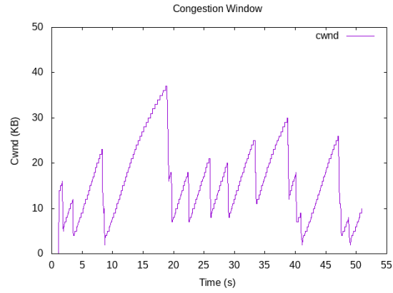
(a) Congestion Window for TCP New Reno
