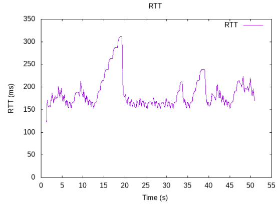
(b) RTT for TCP New Reno.
