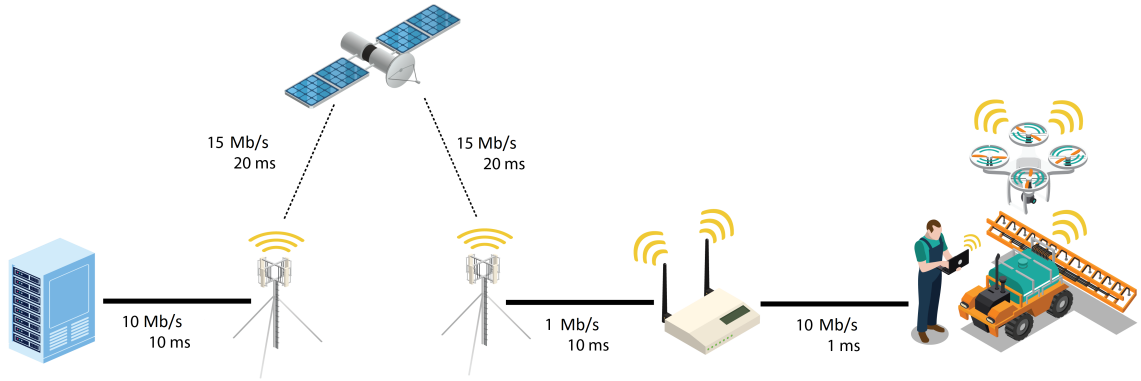
Fig. 2. Topology of the Network.
