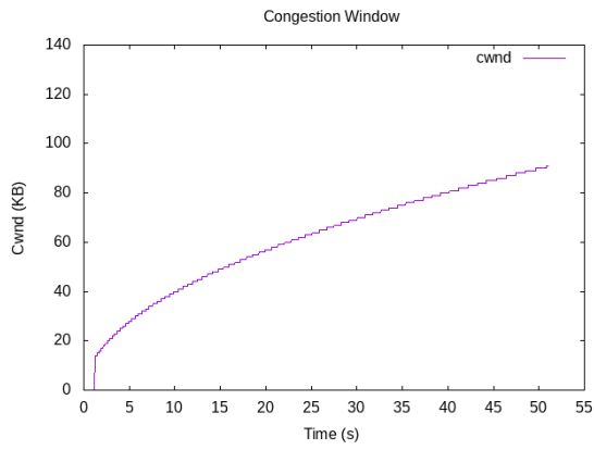
(e) Congestion Window for TCP Westwood.
